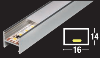
smartLED 1416
