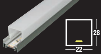
smartLED U2822
